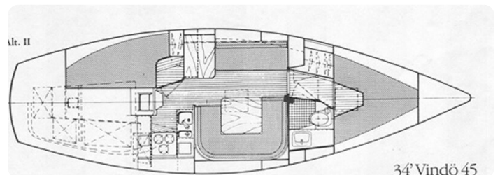
Layout Thula
