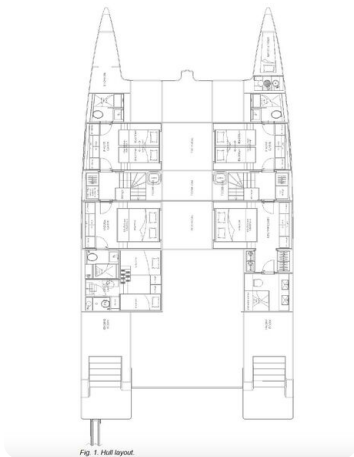
Fig. 1. Hull layout.
