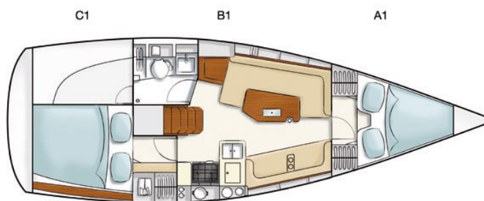
Layout Hanse 320
