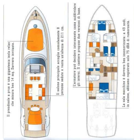
Alalunga Open 85 Sport X Layout
